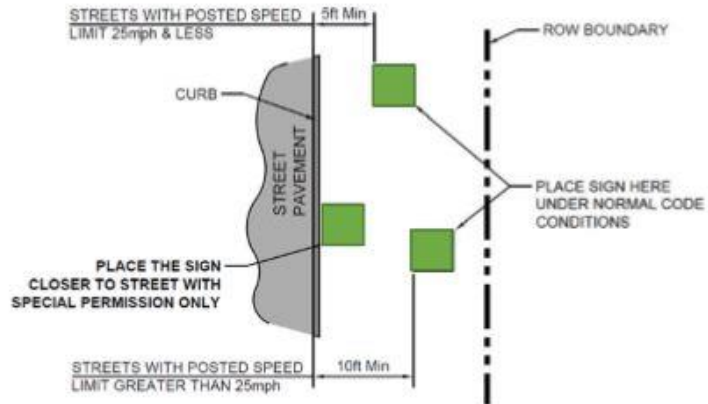
General Code Placement Requirements
